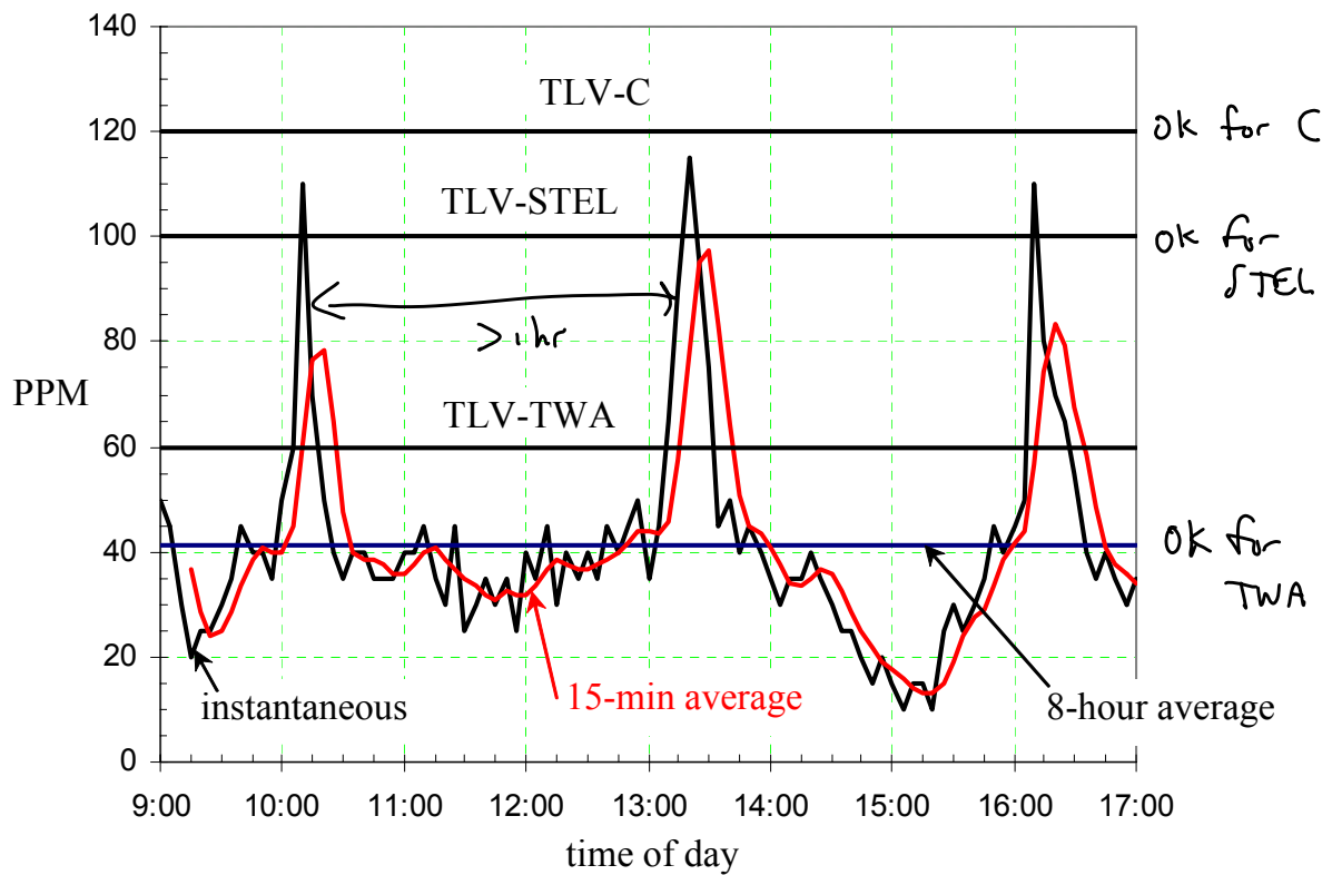
Figure 3.1 Instantaneous and running 15-minute average mol fraction of a contaminant compared to ACGIH standards for an 8-hour work day.
