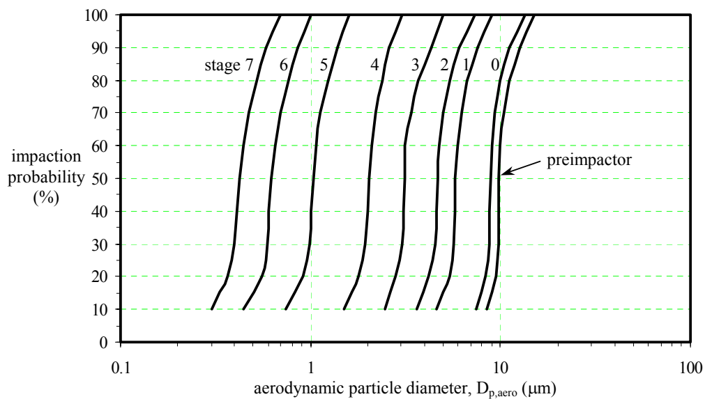
Figure 9.8 Particle collection efficiency for each stage of an Andersen eight-stage, 1 ACFM ambient air sampler with preimpactor (redrawn from Andersen Instruments, Inc.).
