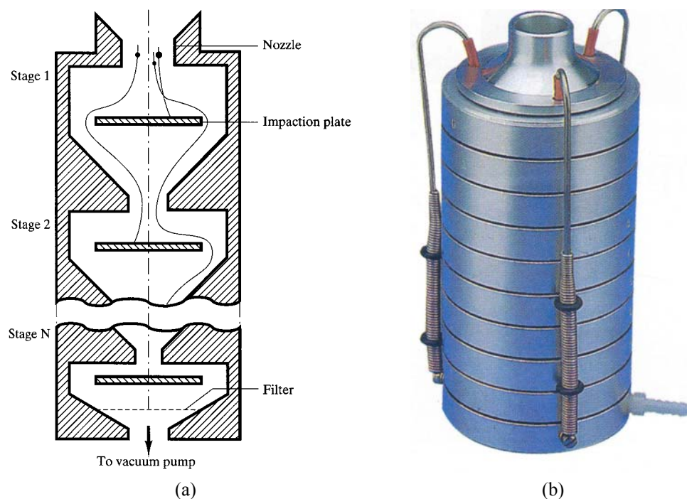
Figure 9.7 Cascade impactor: (a) schematic diagram, showing trajectories of particles of three different diameters (adapted from Willeke and Baron, 1993); (b) Andersen eight-stage, non-viable, 1 ACFM ambient air sampler (from Andersen Instruments Inc.).
