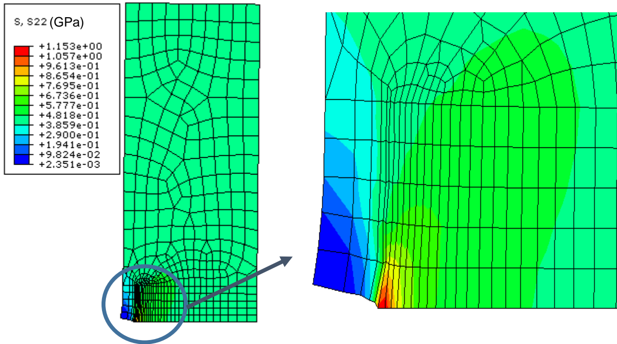
Figure 1: Global 10 S22 plot with focused on crack region
