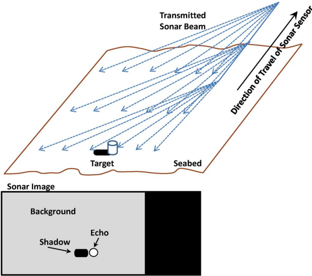
Fig. 1. Illustration of the operation of a typical sidescan sonar. The transmitted sonar beam on the left side of the platform is shown here. A similar sonar beam on the right side of the platform is not shown. Reflections of the sonar beam from the objects on the seabed are also not shown in this figure for clarity of presentation.
