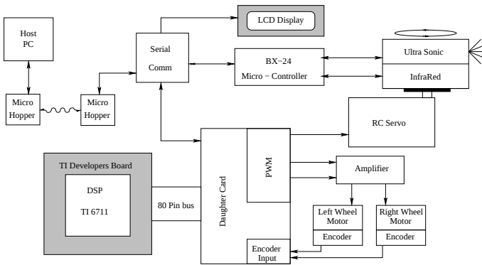
Fig. 3. Hardware diagram of multi-robot testbed.
