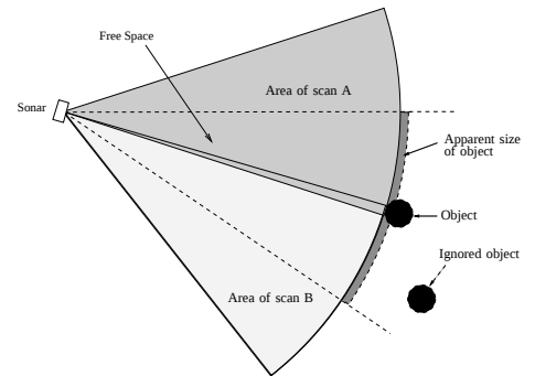
Fig. 5. As a result of the wide beam angle (i) distant objects are not observed and (ii) the 'size' of an object is increased.
